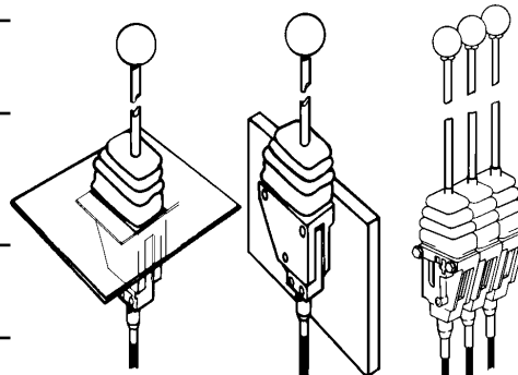
Flush Mounting
